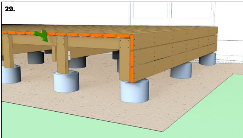
SURFACE TREATMENT
